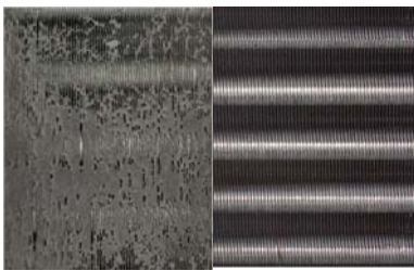
Actual coil image before and after AerisGuard Restoration
